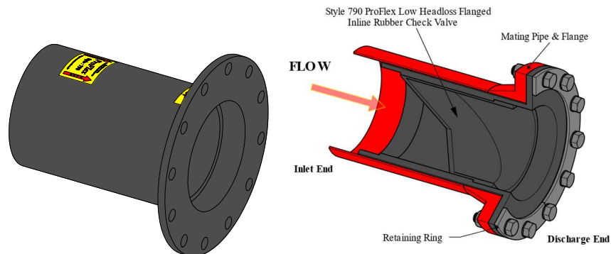
Figure 7: ProFlex Style 790 Low Head Loss Flanged In-Line Rubber Check Valve
