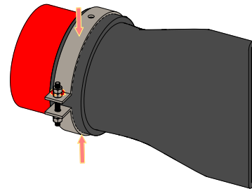
Figure 17: Style 730/731 Installation Step 3
