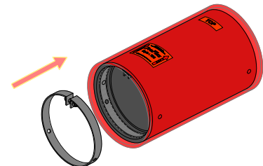
Figure 24: Style 790 Installation Step 2
