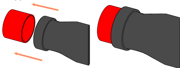
Figure 15: Style 730/731 Installation Step 1
