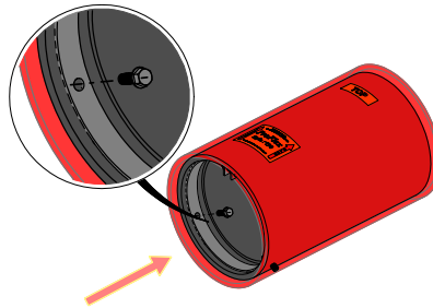
Figure 32: Style 790 Anchor Bolt/Pin Installation
