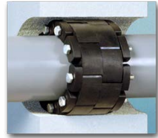
Pipe Penetration Seals
