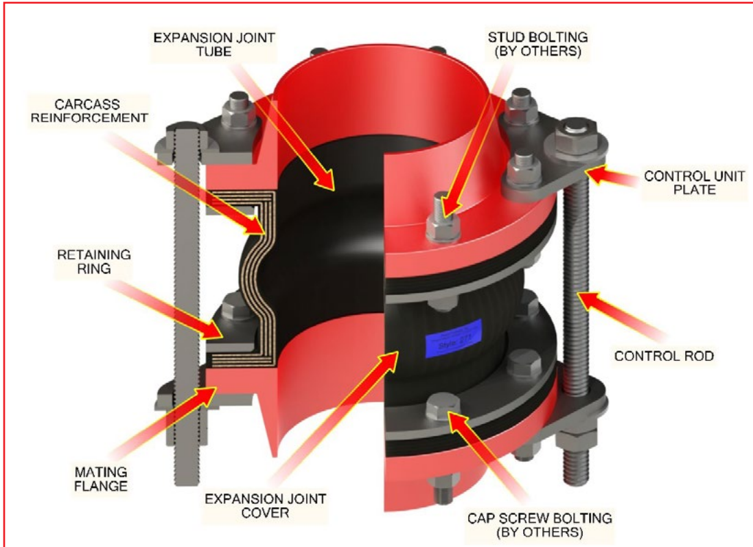
Shown as 271 Single Arch Design with Limit Rod (Figure 1)
