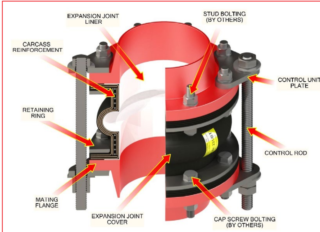
Shown as 231/ET Single Arch Design with Limit Rod (Figure 1)
