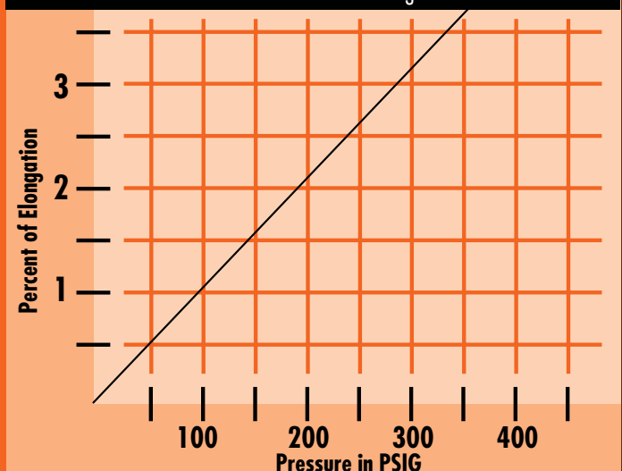
Pressure-Elongation Curve
