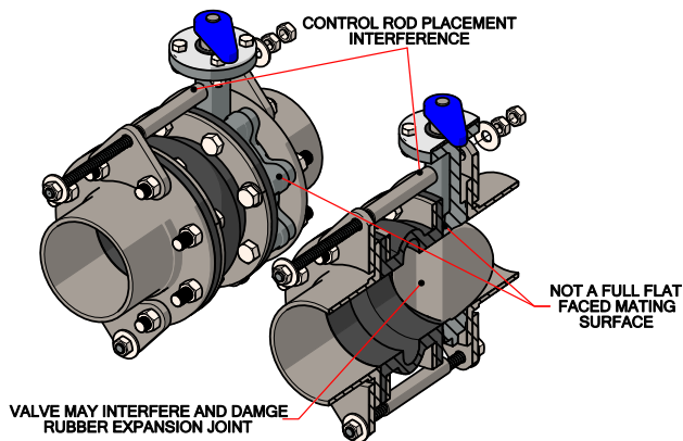
Figure 9: Adjacent Equipment Precaution
