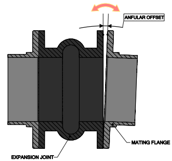
Figure 7: Angular Misalignment
