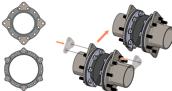
Figure 16: Attach Control Rod Plates to Assembly
