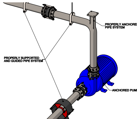
Figure 4: Anchored/Supported System
